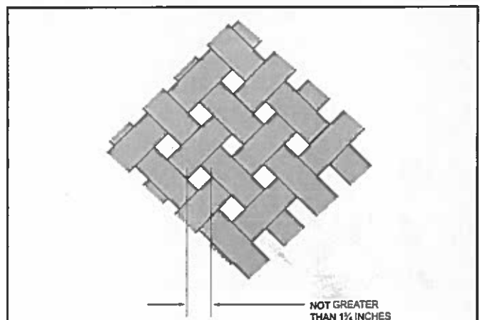
Commentary Figure 305.2.8 MAXIMUM OPENING WIDTH IN BARRIERS BUILT WITH DIAGONAL MEMBERS
