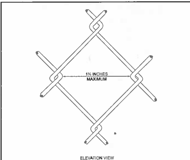
Commentary Figure 305.2.7 MAXIMUM OPENING WIDTH IN BARRIERS BUILT WITH CHAIN LINK FENCING
